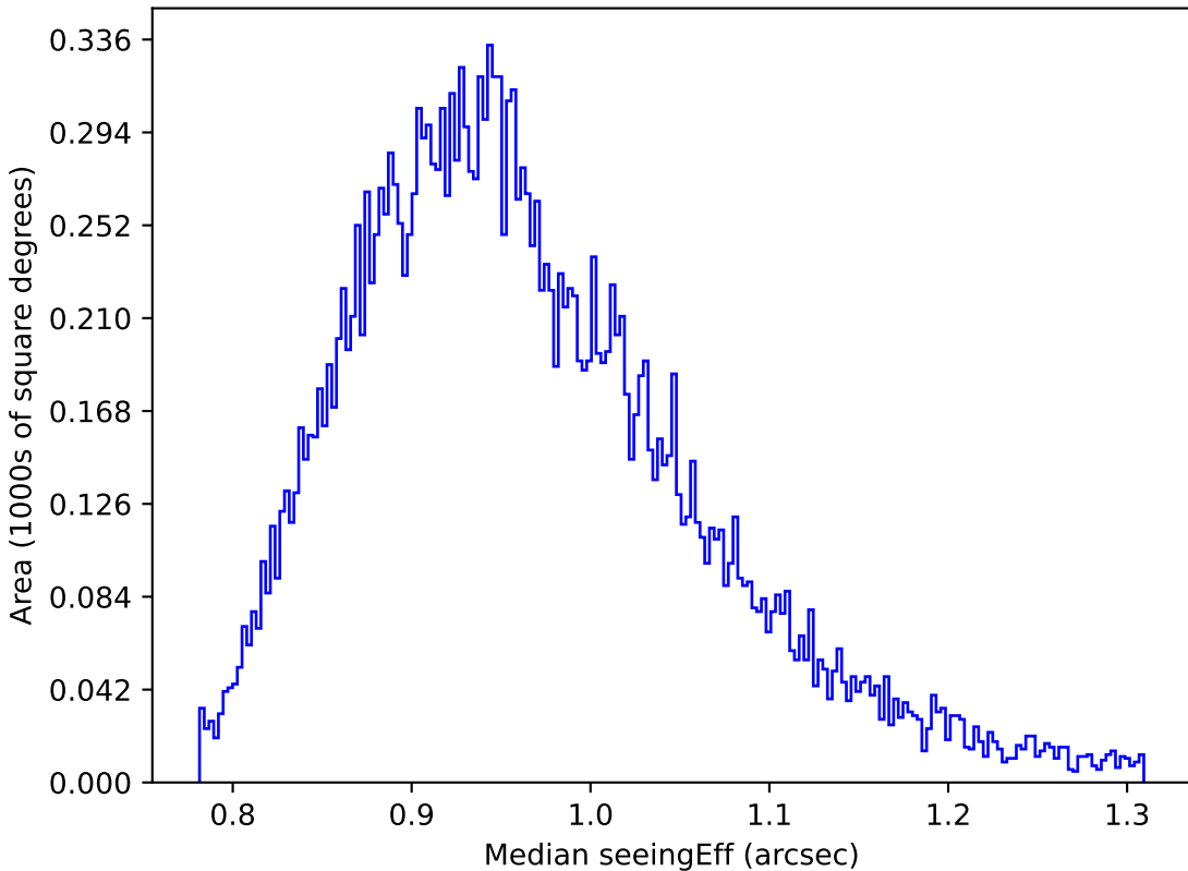
too_5_4v3.4_10yrs Yr 1 y band: Median seeingEff
