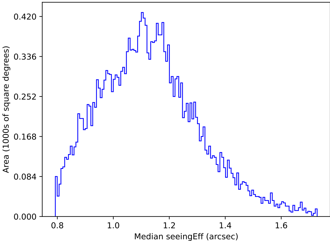
too_5_4v3.4_10yrs Yr 1 u band: Median seeingEff
