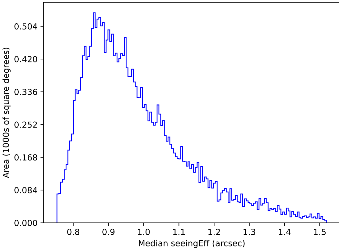
too_5_4v3.4_10yrs Yr 1 r band: Median seeingEff
