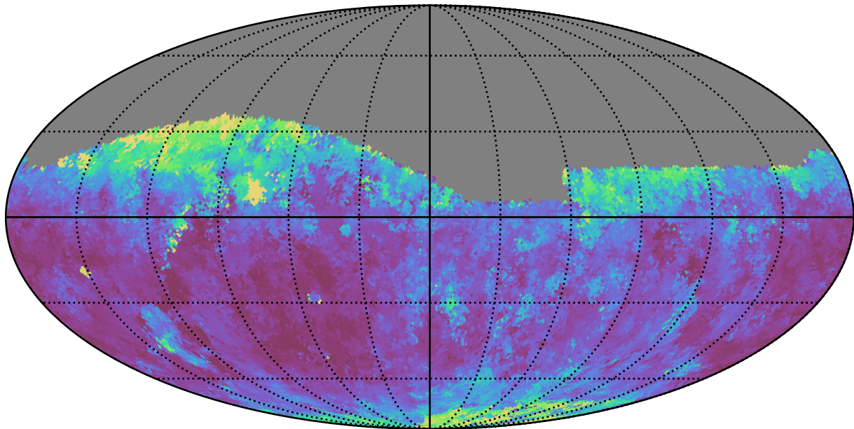
too_5_4v3.4_10yrs Yr 1 i band: Median seeingEff
