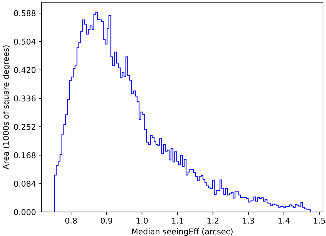
too_5_4v3.4_10yrs Yr 1 i band: Median seeingEff
