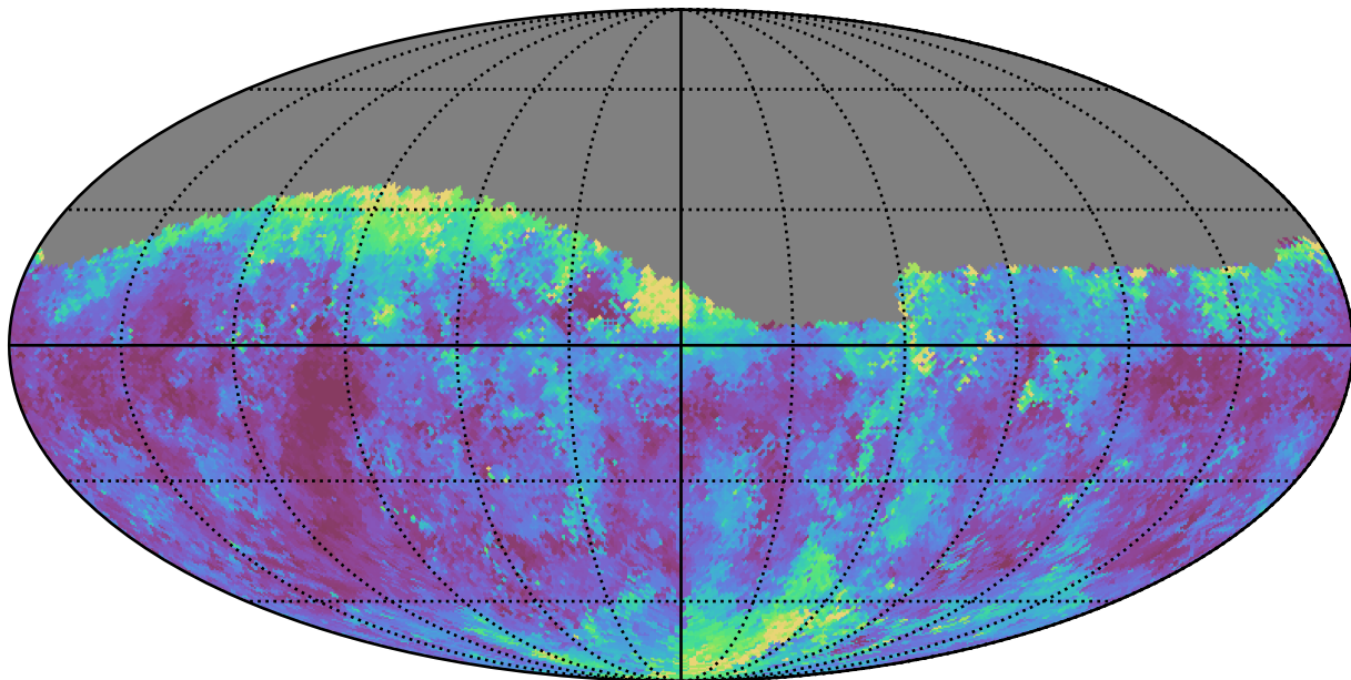
too_5_4v3.4_10yrs Yr 1 g band: Median seeingEff
