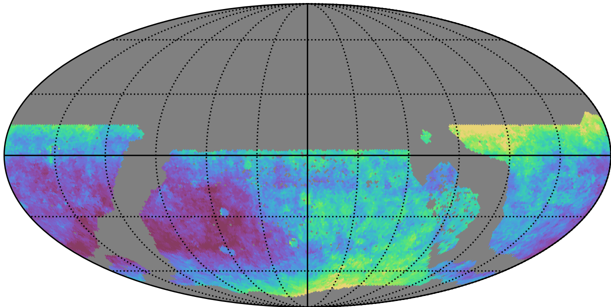
too_5_4v3.4_10yrs WFD z band: Median seeingEff
