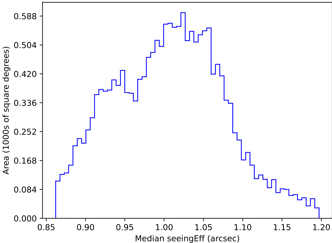
too_5_4v3.4_10yrs WFD z band: Median seeingEff
