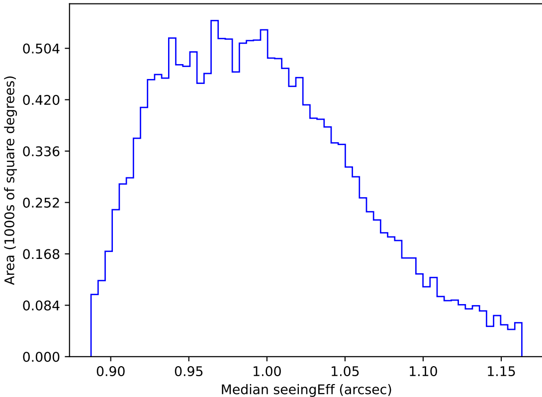
too_5_4v3.4_10yrs WFD y band: Median seeingEff
