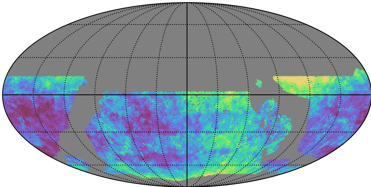
too_5_4v3.4_10yrs WFD u band: Median seeingEff
