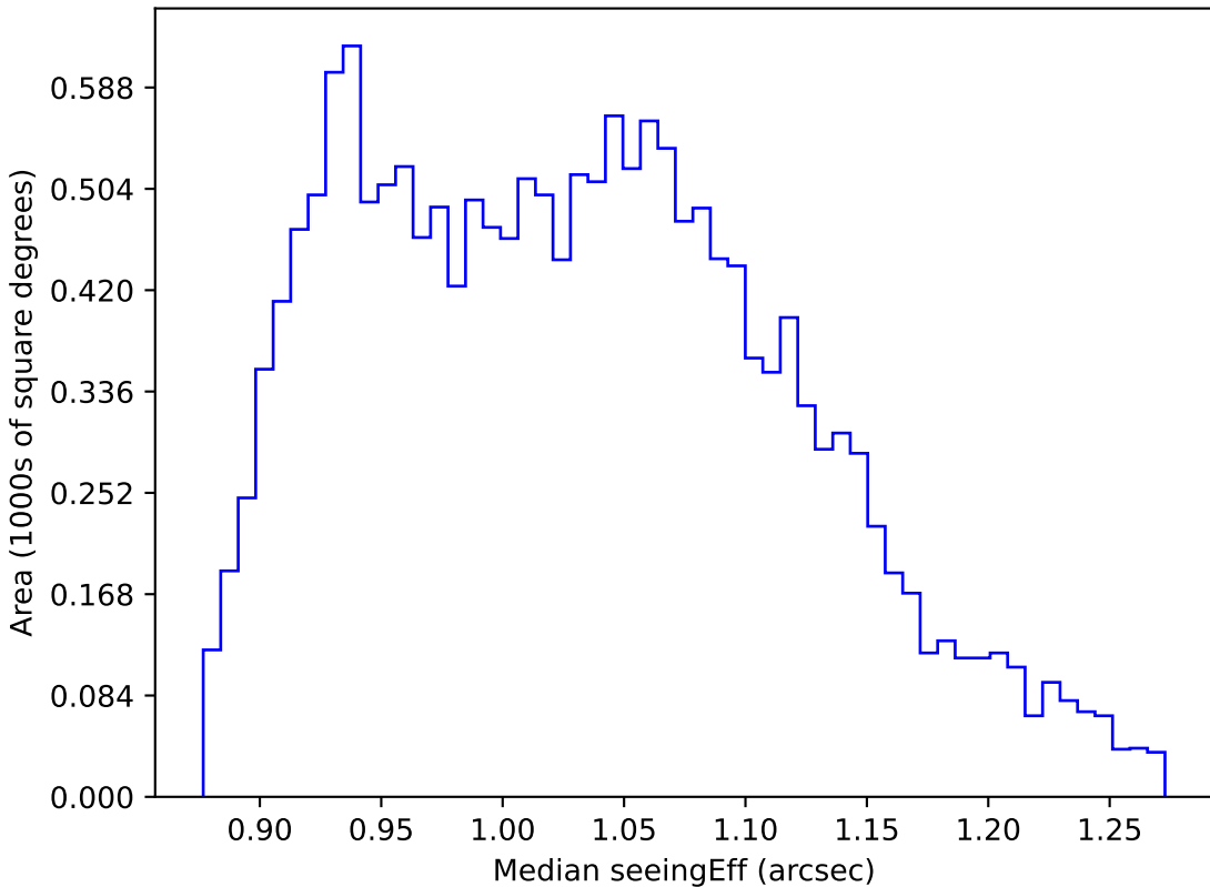
too_5_4v3.4_10yrs WFD r band: Median seeingEff
