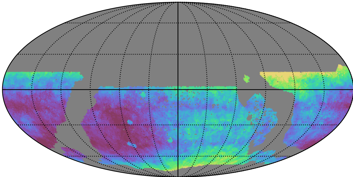
too_5_4v3.4_10yrs WFD i band: Median seeingEff
