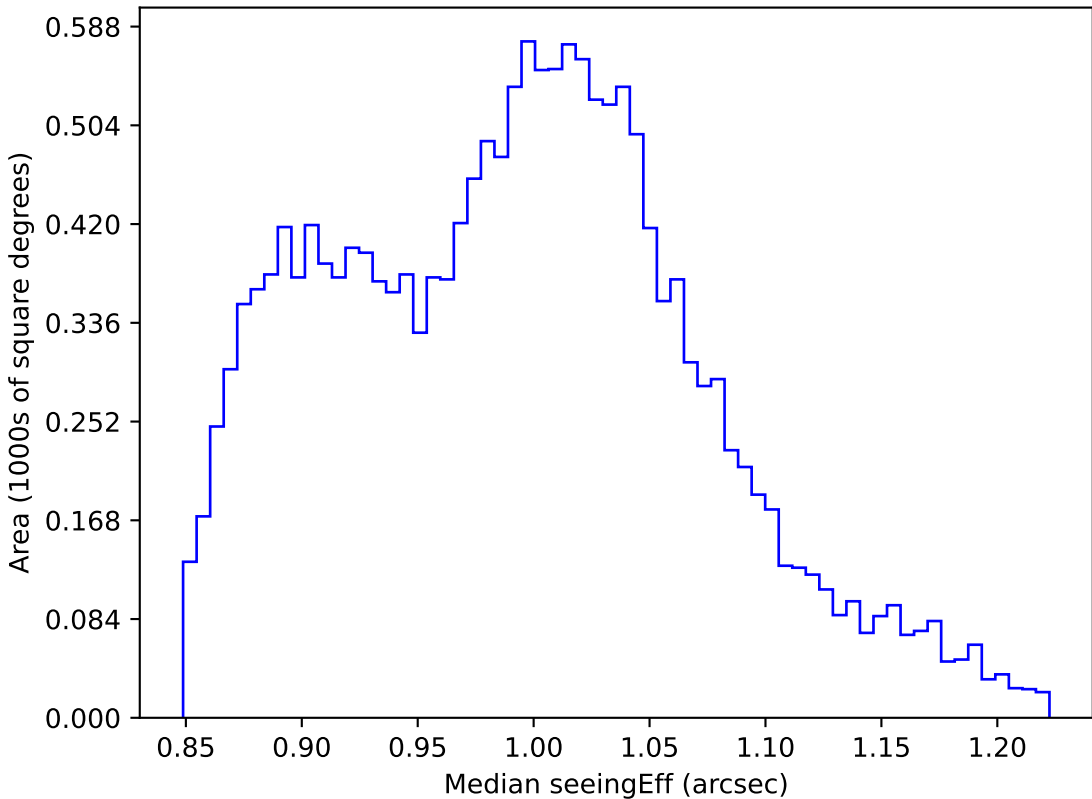
too_5_4v3.4_10yrs WFD i band: Median seeingEff
