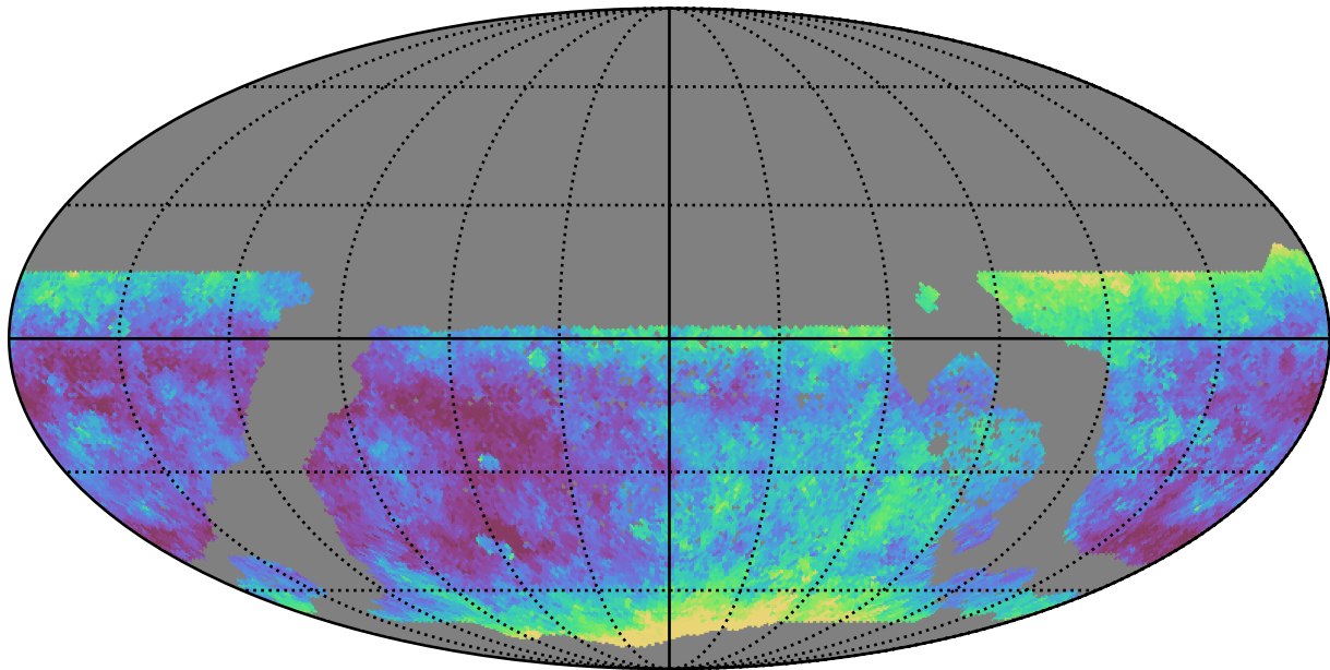
too_5_4v3.4_10yrs WFD g band: Median seeingEff
