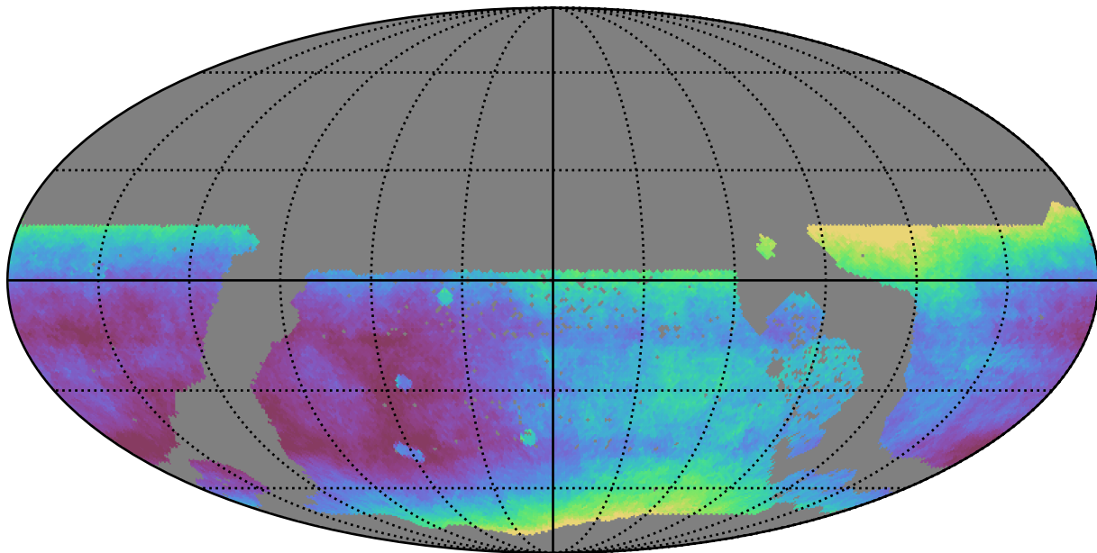
too_5_4v3.4_10yrs WFD all bands: Median seeingEff
