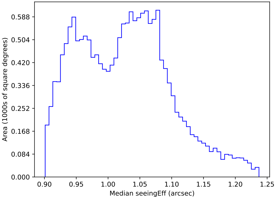
too_5_4v3.4_10yrs WFD all bands: Median seeingEff
