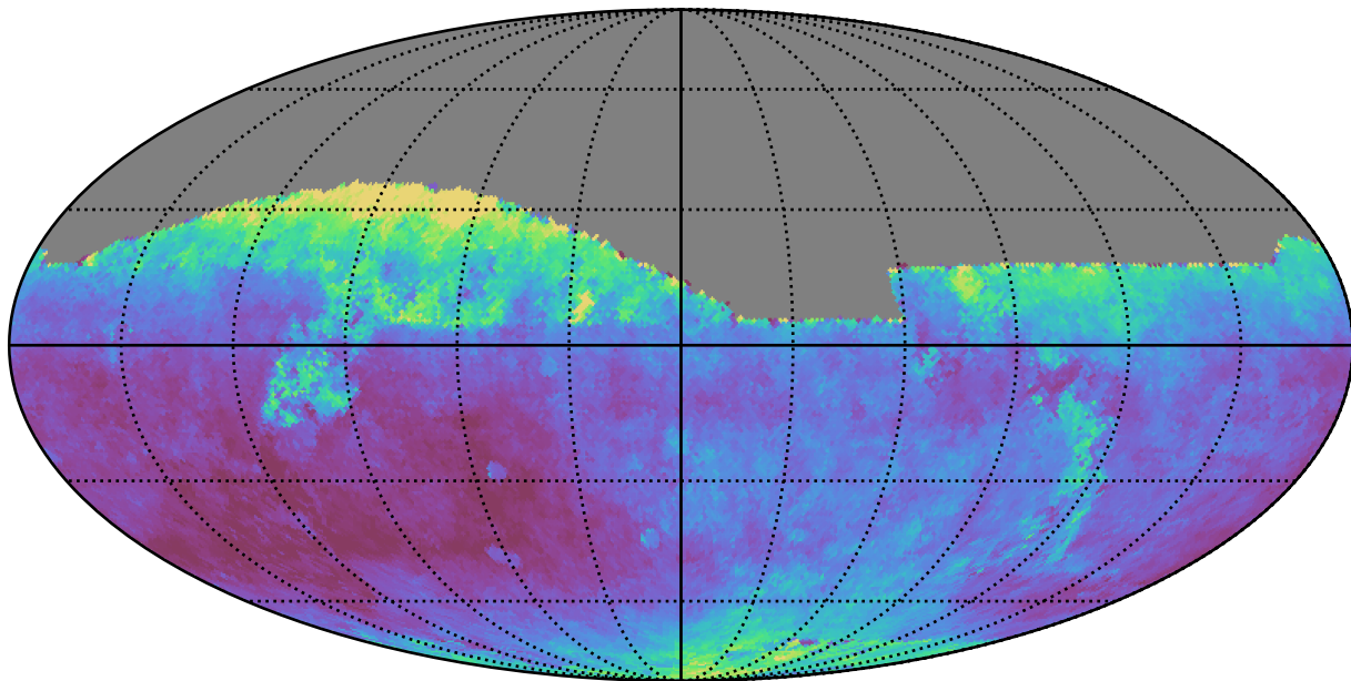
too_5_4v3.4_10yrs All sky z band: Median seeingEff
