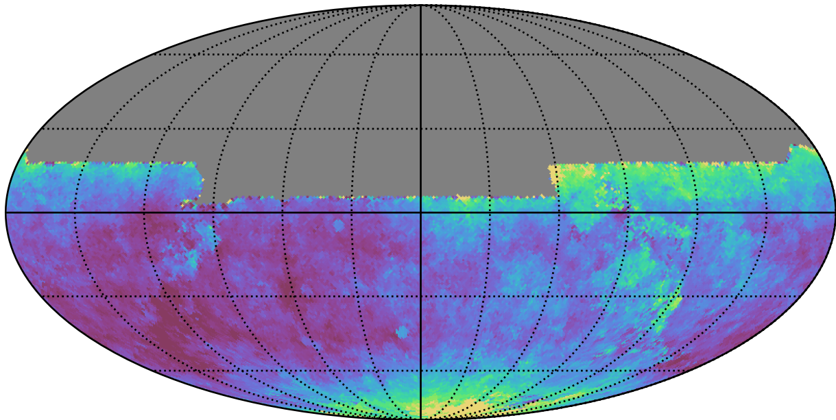
too_5_4v3.4_10yrs All sky y band: Median seeingEff
