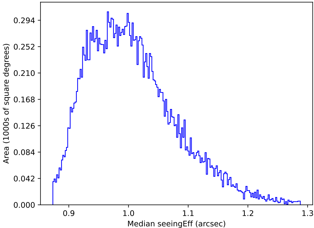
too_5_4v3.4_10yrs All sky y band: Median seeingEff
