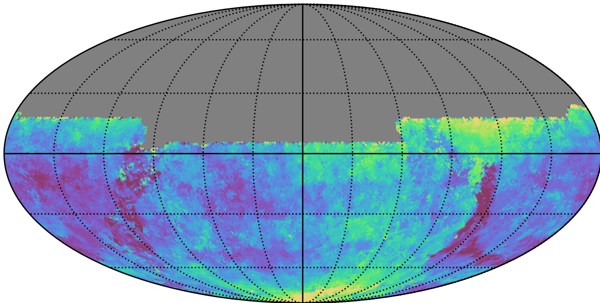
too_5_4v3.4_10yrs All sky u band: Median seeingEff
