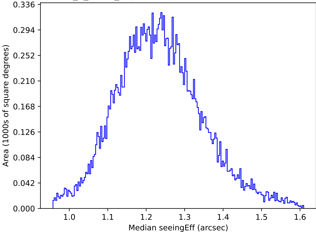
too_5_4v3.4_10yrs All sky u band: Median seeingEff
