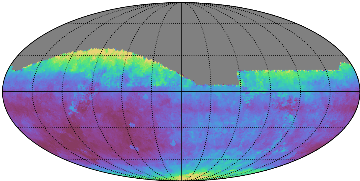
too_5_4v3.4_10yrs All sky i band: Median seeingEff
