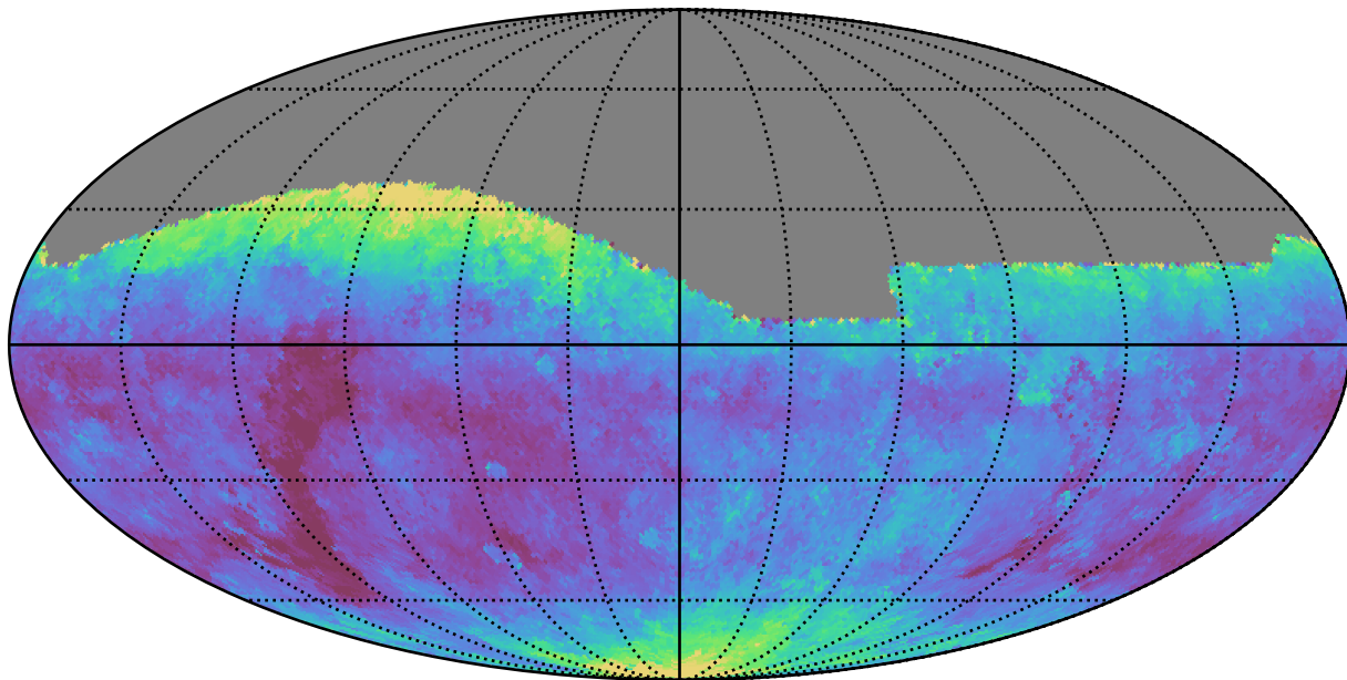
too_5_4v3.4_10yrs All sky g band: Median seeingEff
