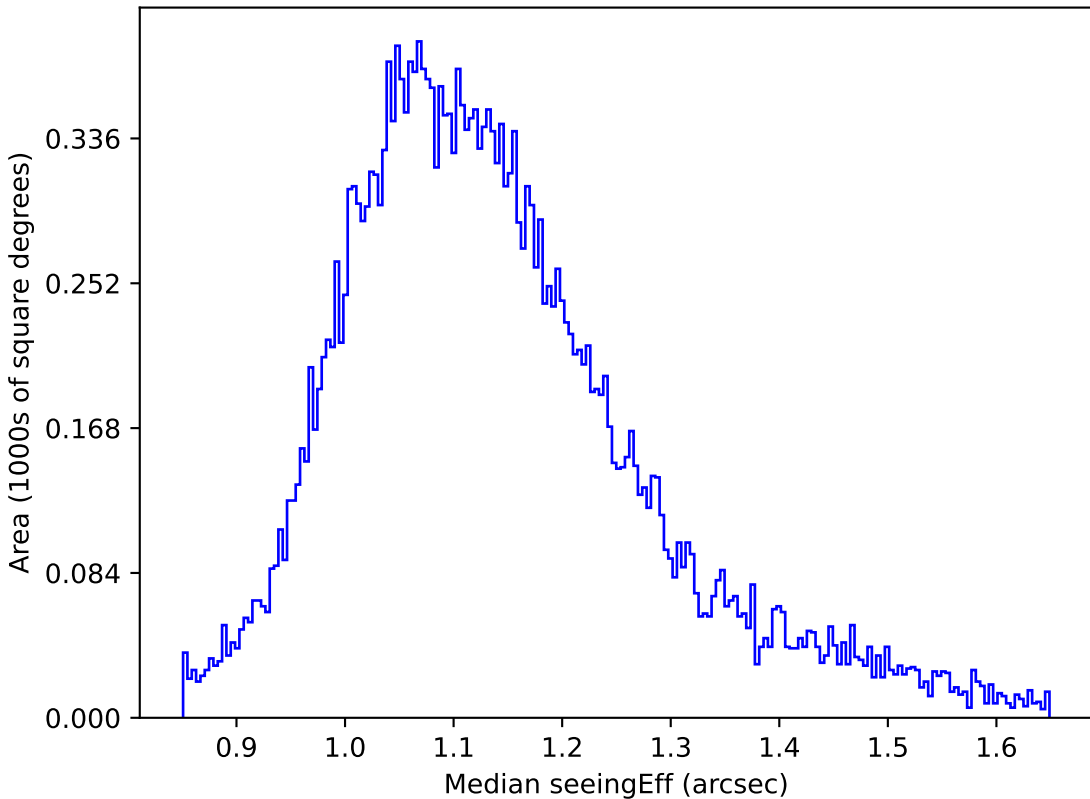
too_5_4v3.4_10yrs All sky g band: Median seeingEff
