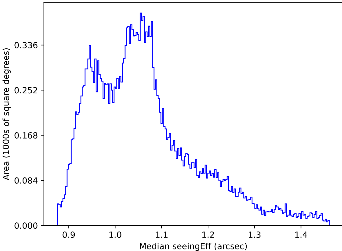
too_5_4v3.4_10yrs All sky all bands: Median seeingEff
