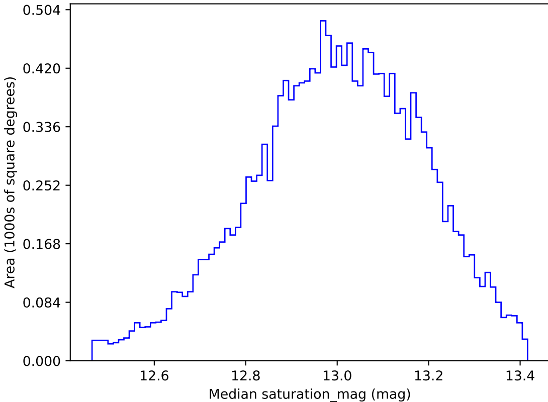
too_5_4v3.4_10yrs WFD u band: Median saturation_mag
