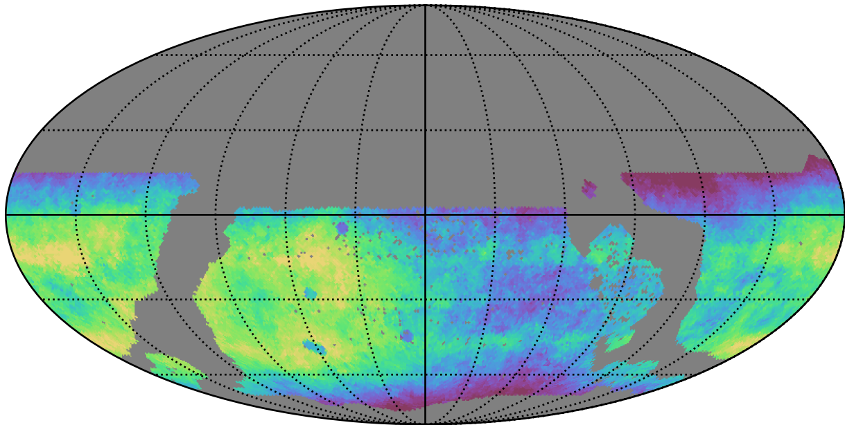
too_5_4v3.4_10yrs WFD r band: Median saturation_mag
