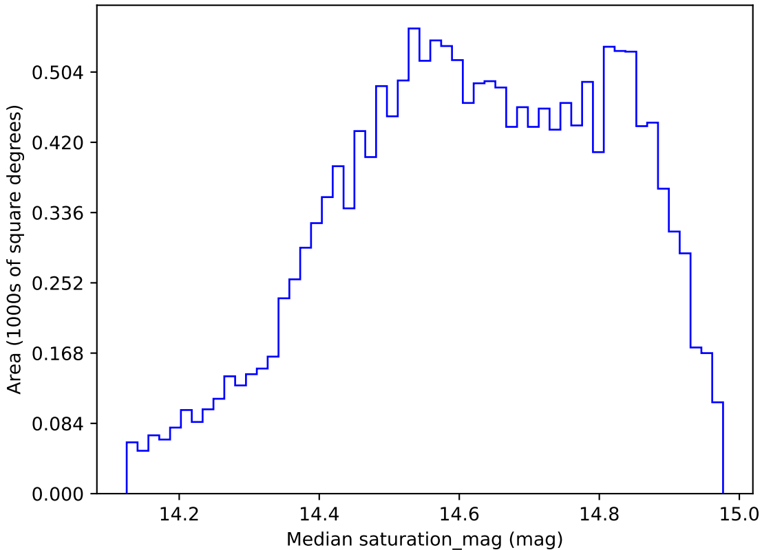
too_5_4v3.4_10yrs WFD r band: Median saturation_mag
