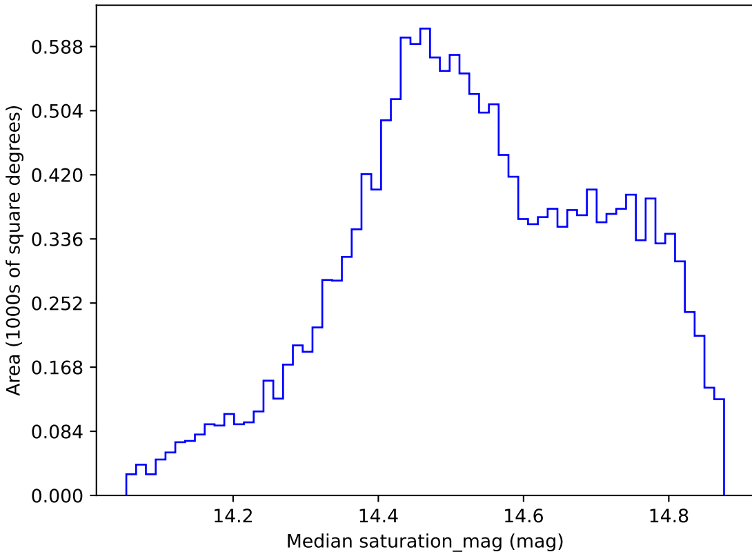
too_5_4v3.4_10yrs WFD i band: Median saturation_mag
