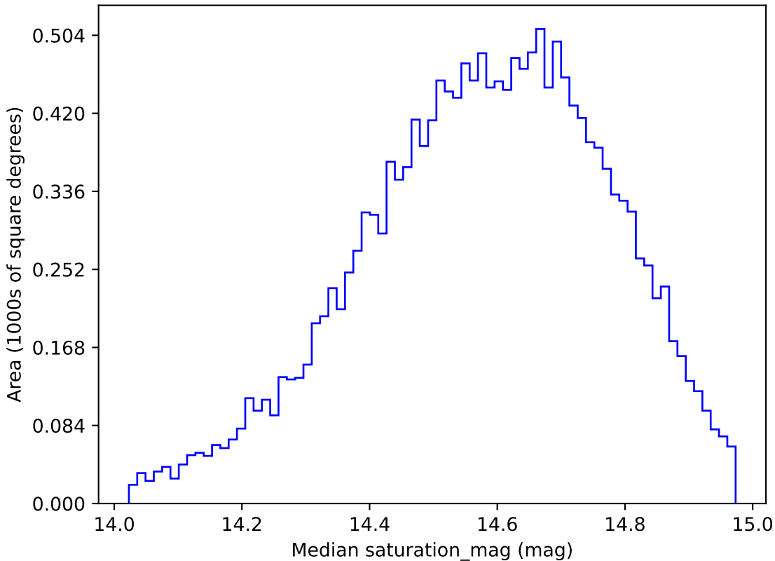
too_5_4v3.4_10yrs WFD g band: Median saturation_mag
