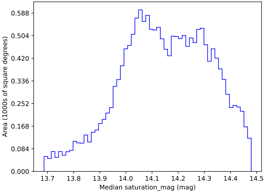
too_5_4v3.4_10yrs WFD all bands: Median saturation_mag
