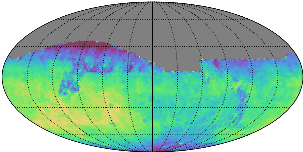
too_5_4v3.4_10yrs All sky z band: Median saturation_mag
