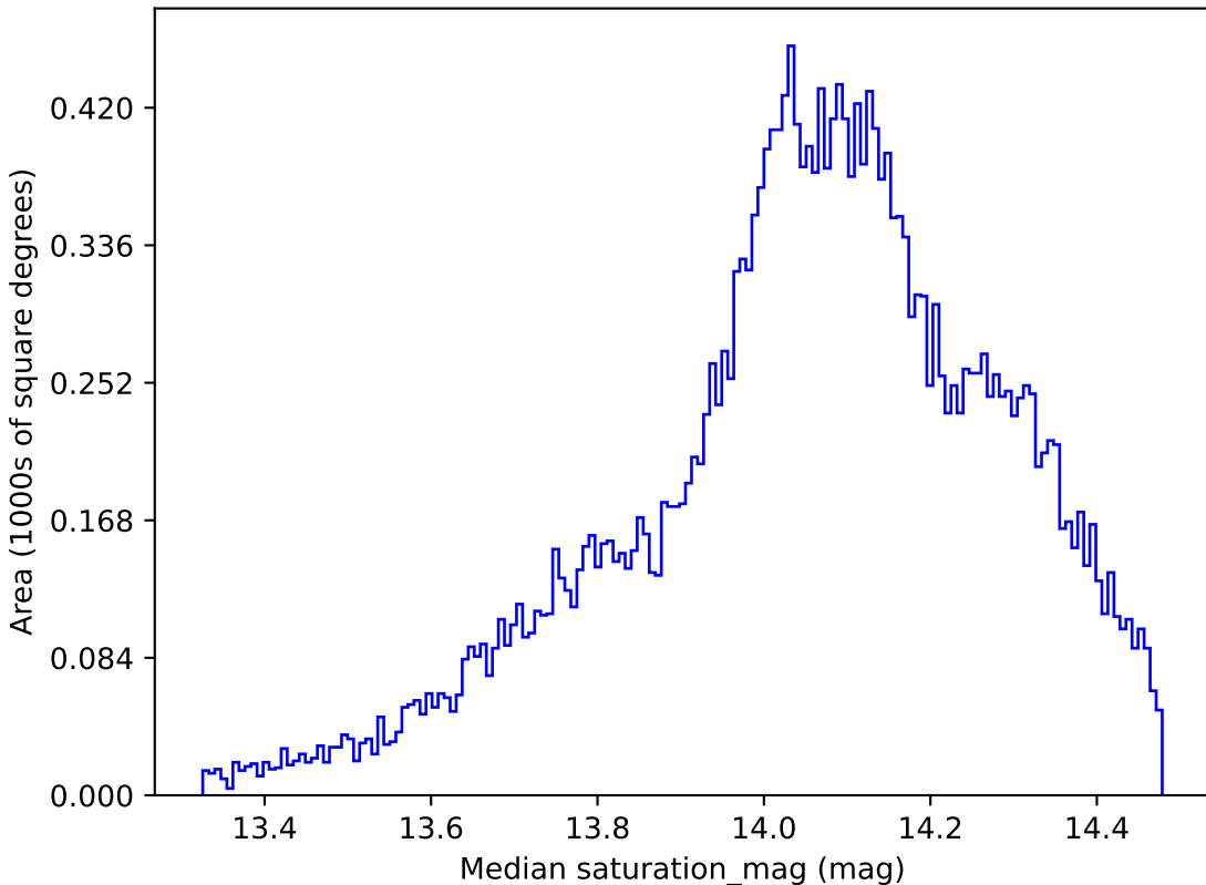
too_5_4v3.4_10yrs All sky z band: Median saturation_mag
