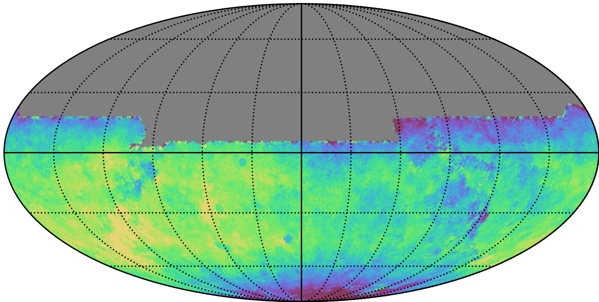
too_5_4v3.4_10yrs All sky y band: Median saturation_mag
