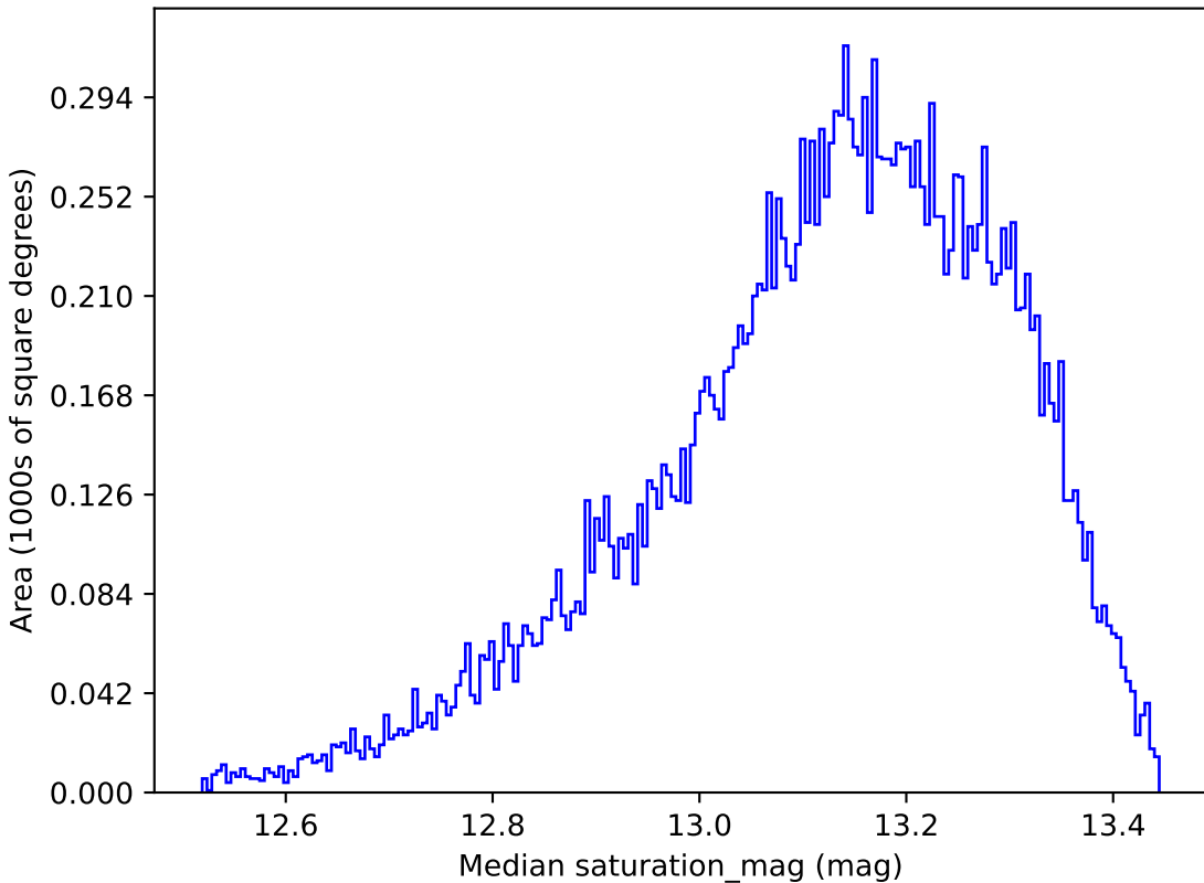
too_5_4v3.4_10yrs All sky y band: Median saturation_mag
