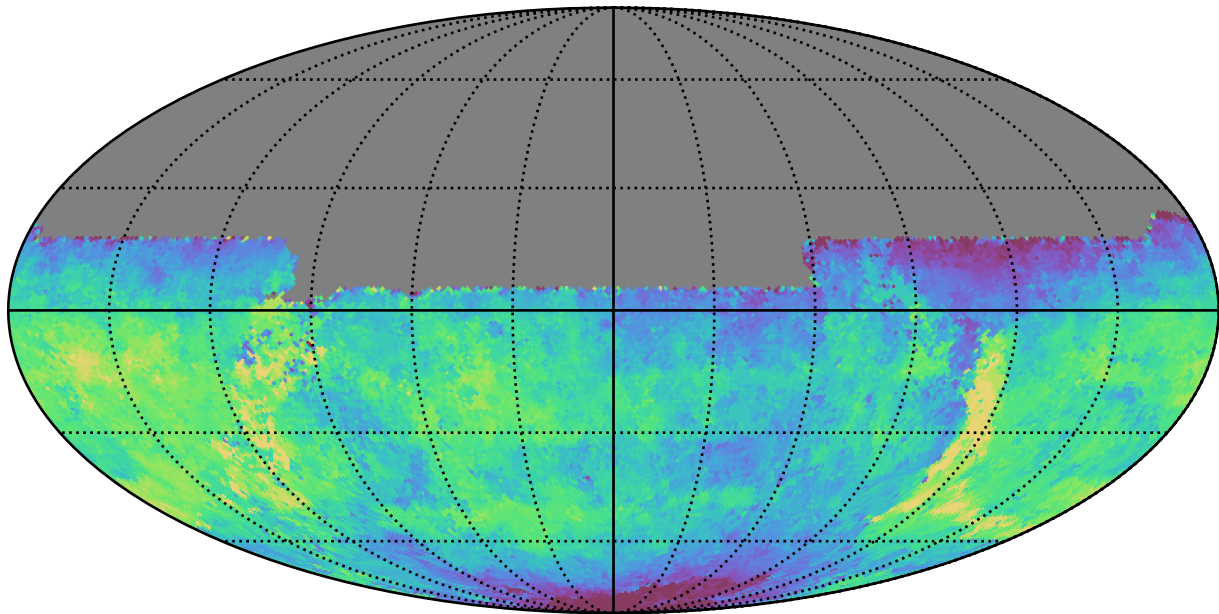
too_5_4v3.4_10yrs All sky u band: Median saturation_mag
