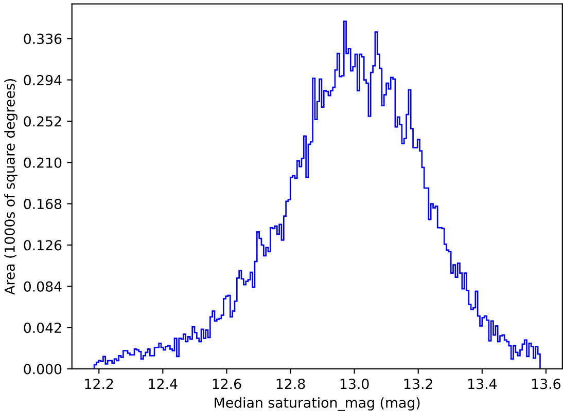
too_5_4v3.4_10yrs All sky u band: Median saturation_mag
