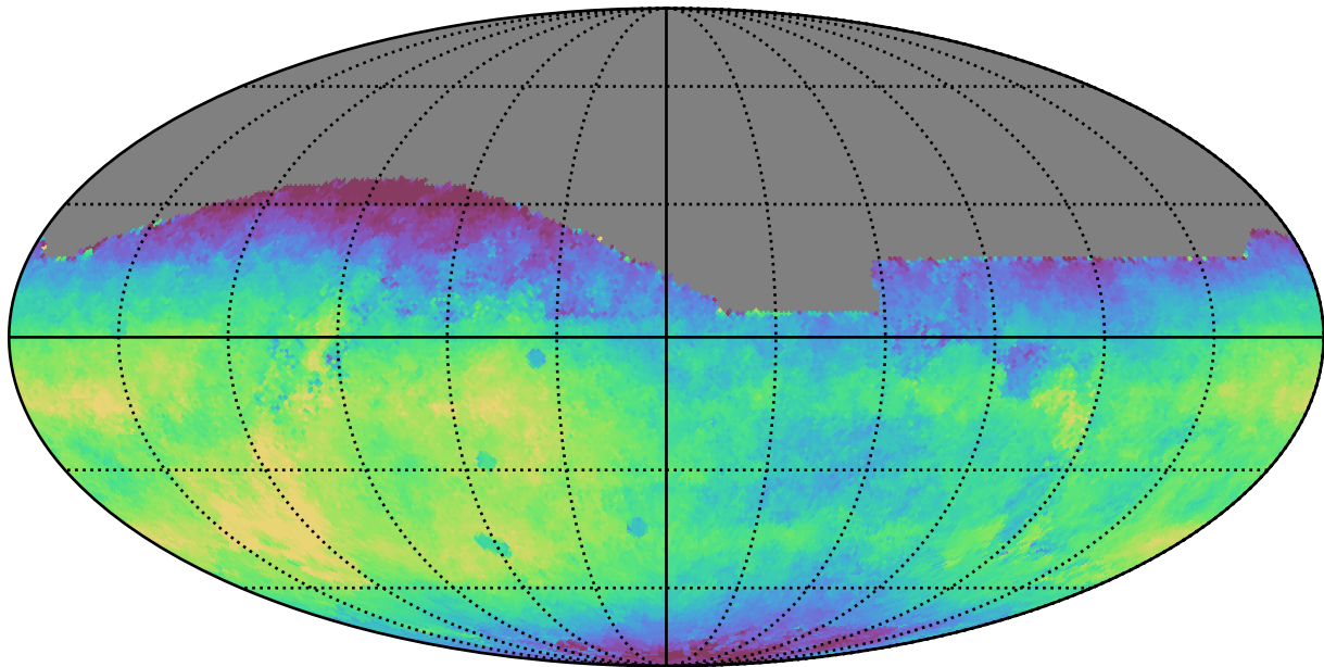
too_5_4v3.4_10yrs All sky r band: Median saturation_mag
