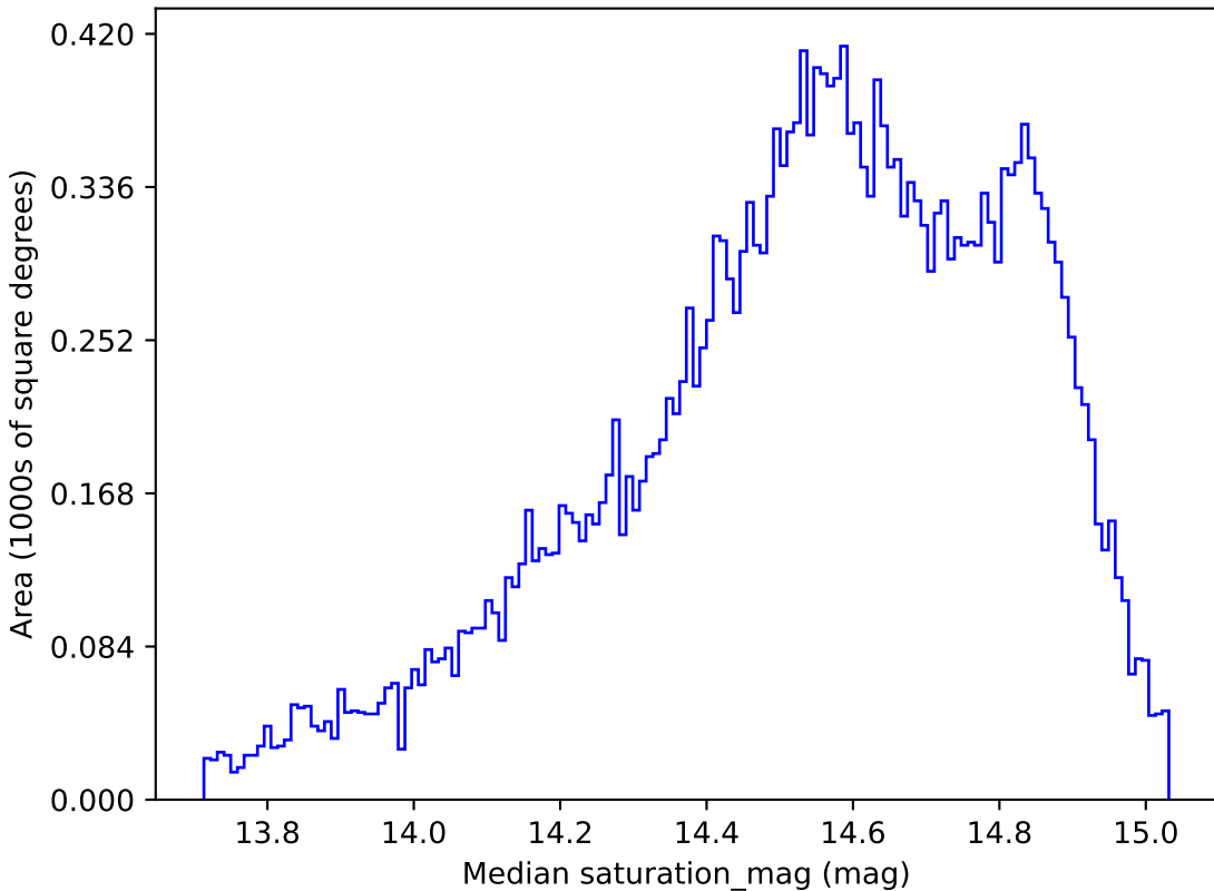
too_5_4v3.4_10yrs All sky r band: Median saturation_mag
