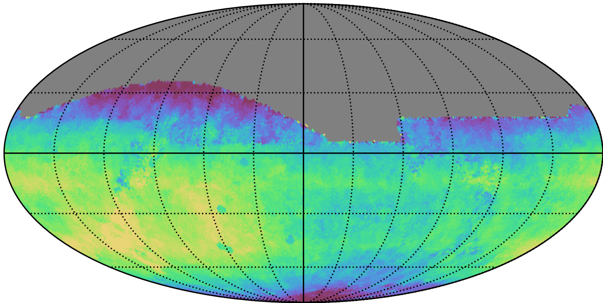
too_5_4v3.4_10yrs All sky i band: Median saturation_mag
