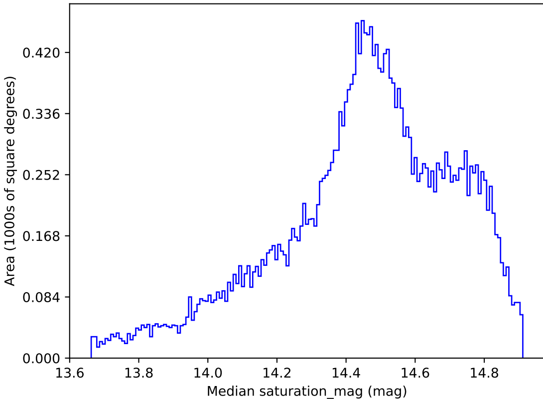
too_5_4v3.4_10yrs All sky i band: Median saturation_mag
