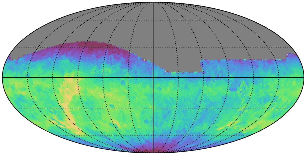
too_5_4v3.4_10yrs All sky g band: Median saturation_mag
