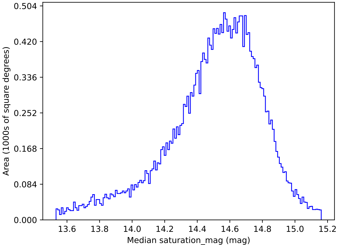
too_5_4v3.4_10yrs All sky g band: Median saturation_mag
