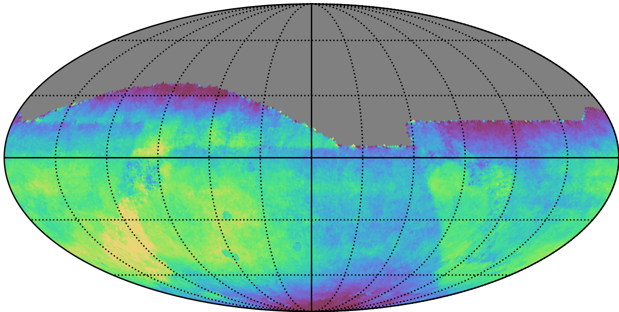
too_5_4v3.4_10yrs All sky all bands: Median saturation_mag
