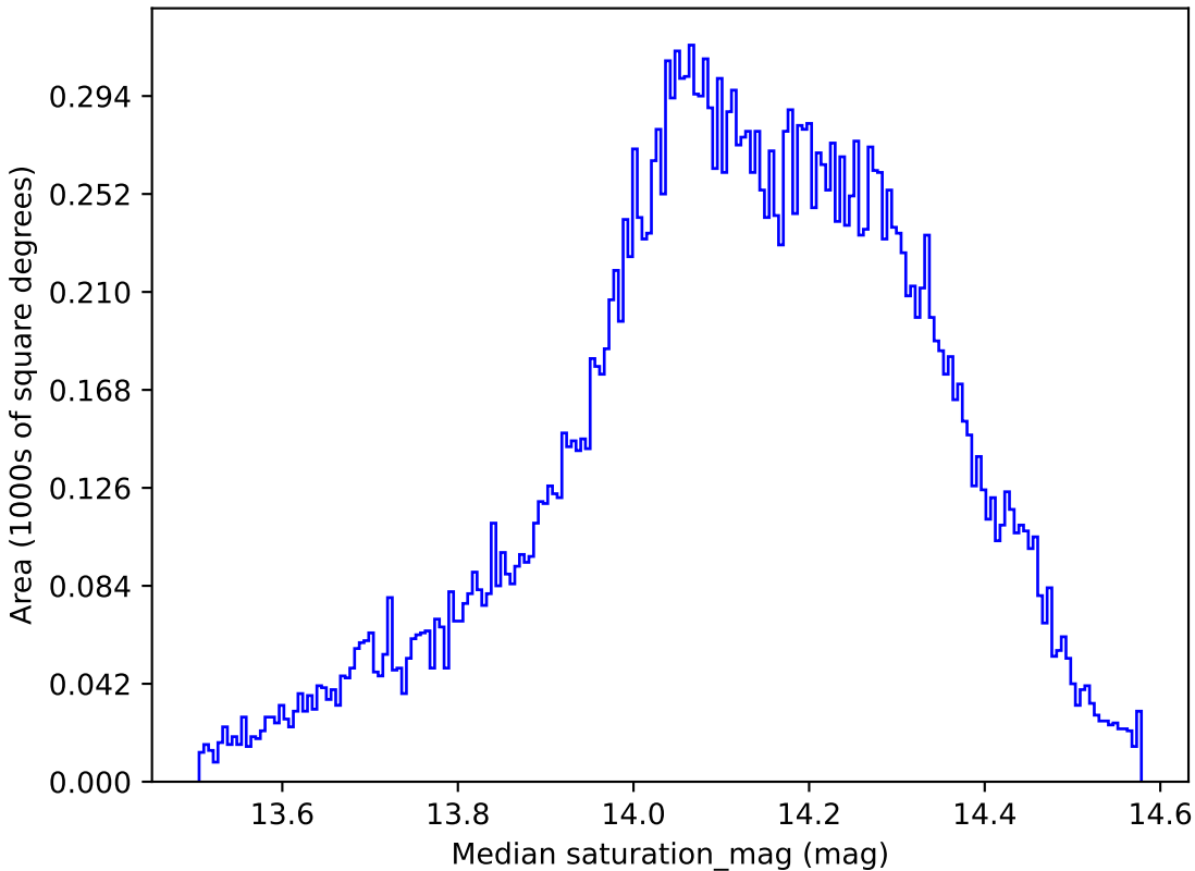
too_5_4v3.4_10yrs All sky all bands: Median saturation_mag
