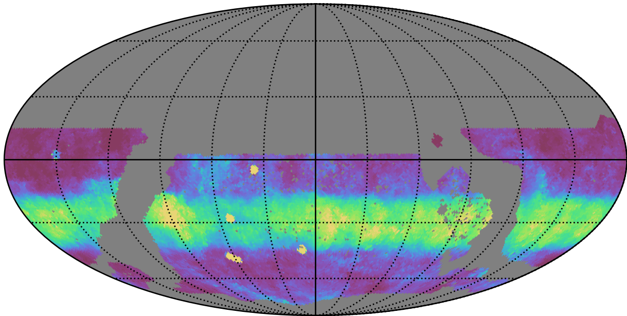
too_5_4v3.4_10yrs WFD z band: Median normairmass
