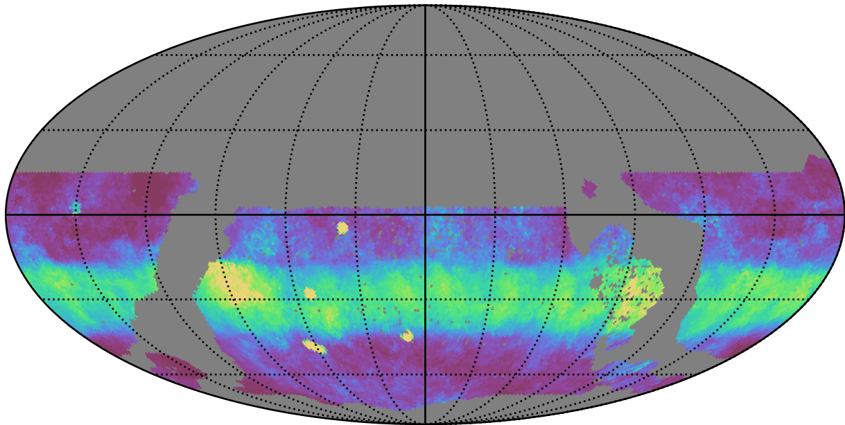
too_5_4v3.4_10yrs WFD y band: Median normairmass
