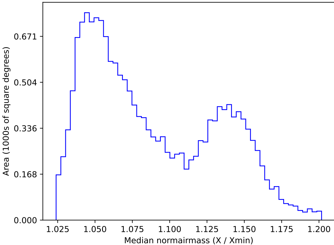
too_5_4v3.4_10yrs WFD y band: Median normairmass
