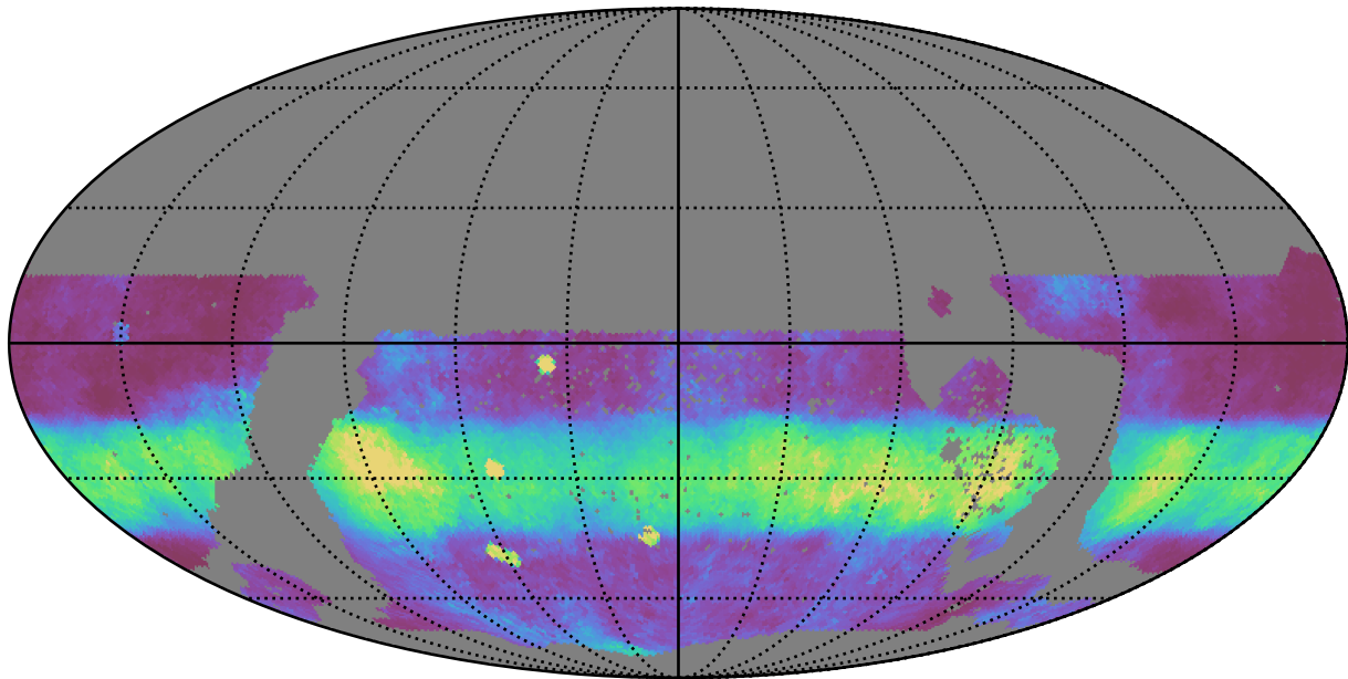
too_5_4v3.4_10yrs WFD r band: Median normairmass
