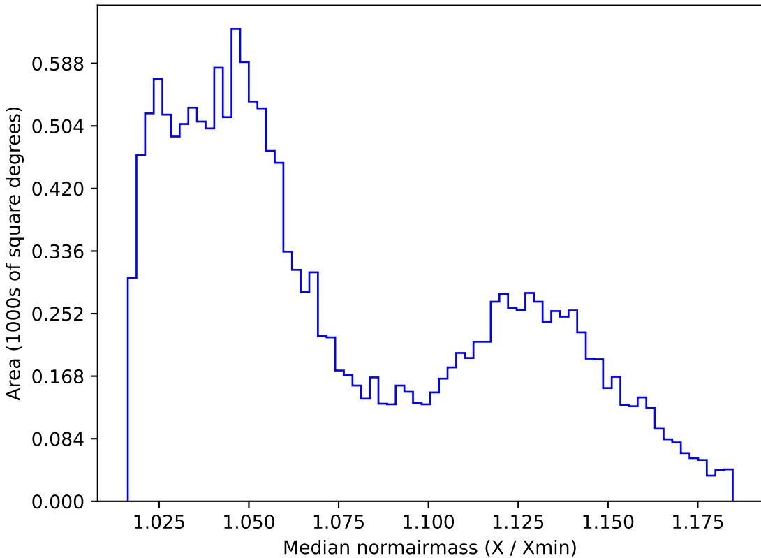
too_5_4v3.4_10yrs WFD r band: Median normairmass
